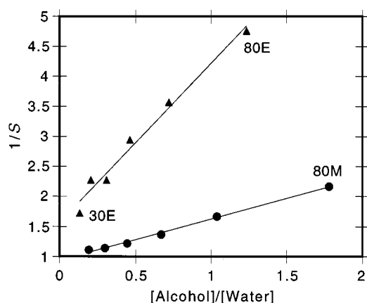
Fig. 3 Plots of 1/S [equation (3)] versus molar ratio of solvents, [\text{alcohol}]/[\text{water}] , for solvolyses of diphenyl phosphorochloridate 1 at 25 °C; S values from Table 6. For ethanol–water: slope = 2.654 \pm 0.183 , intercept = 1.557 \pm 0.116 , r = 0.991 . For methanol–water: slope = 0.688 \pm 0.022 , intercept = 0.939 \pm 0.020 , r = 0.998
