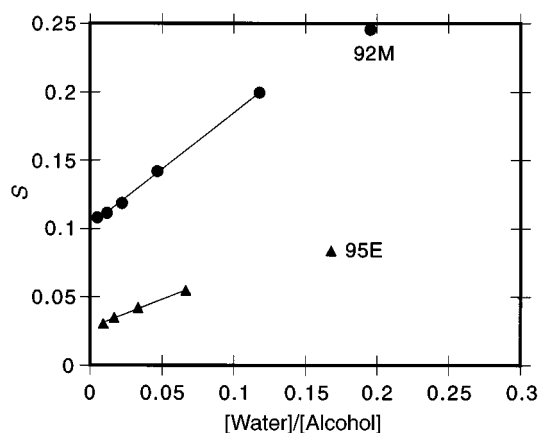
Fig. 4 Plots of S [equation (4)] versus molar ratio of solvents, [\text{water}]/[\text{alcohol}] , for solvolyses of diphenyl phosphorochloridate 1 at 0 °C; S values from Table 6. For ethanol–water: slope = 0.419 \pm 0.023 , intercept = 0.0275 \pm 0.0009 , r = 0.997 . For methanol–water: slope = 0.824 \pm 0.018 , intercept = 0.103 \pm 0.001 , r = 0.999
